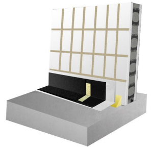
ICF Wall
