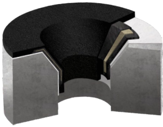
Deck Drain
