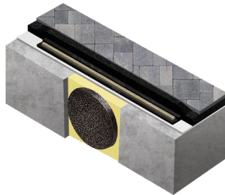
Expansion Joint
