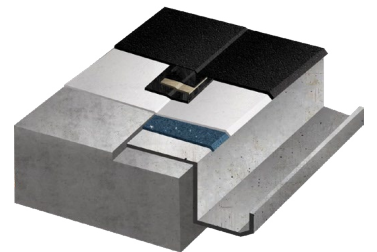
Gutter Transition
